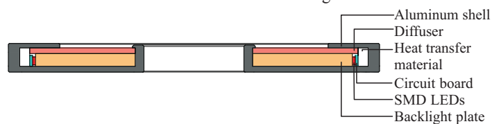
Section Structure Drawing
